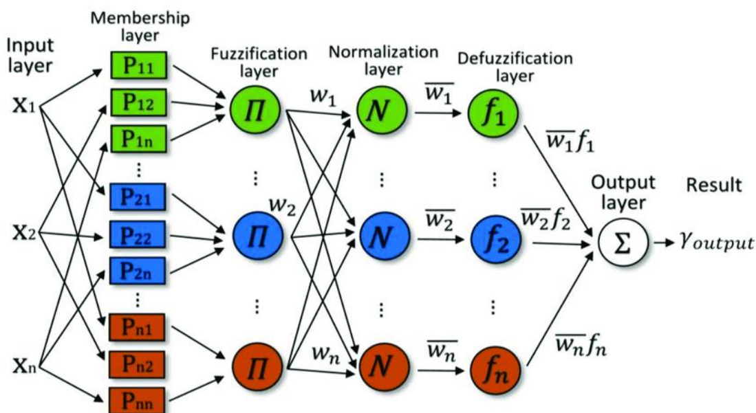
Figure 3. ANFIS five layer structure
