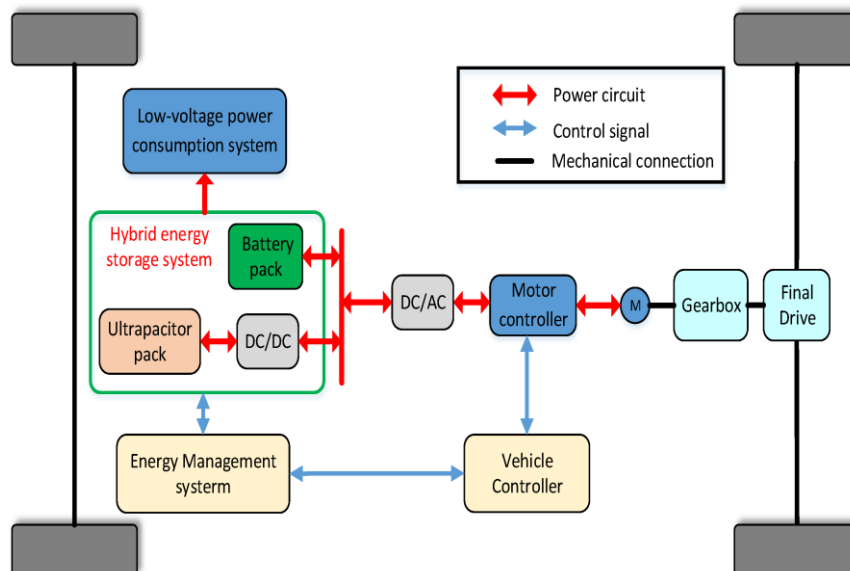
Figure 2. Proposed Hybrid Power Management System
