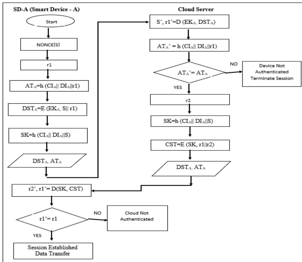
Figure 3: Flowchart of our proposed mechanism
