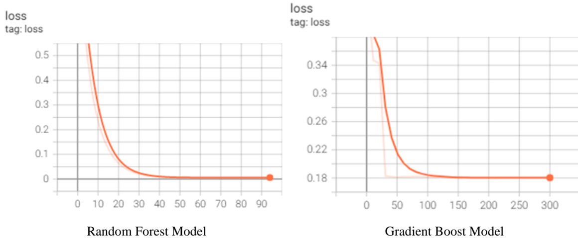
Fig.14: Loss tag
