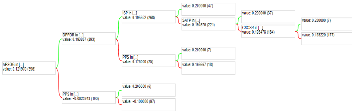
Fig.9: Random Forest Model
