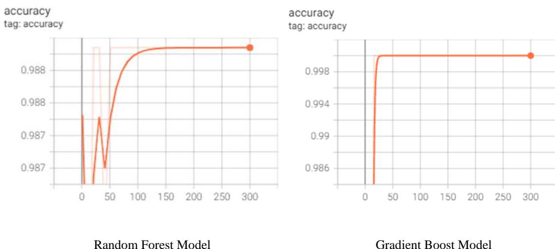
Fig.13: Accuracy tag
