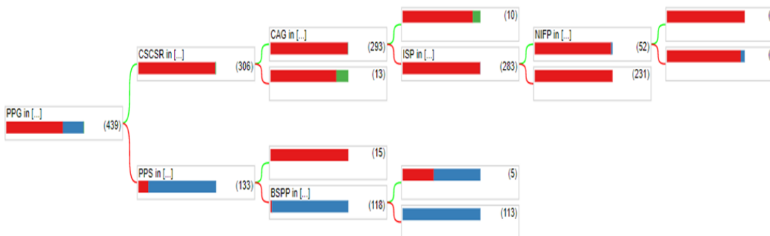
Fig. 11: Cart Model
