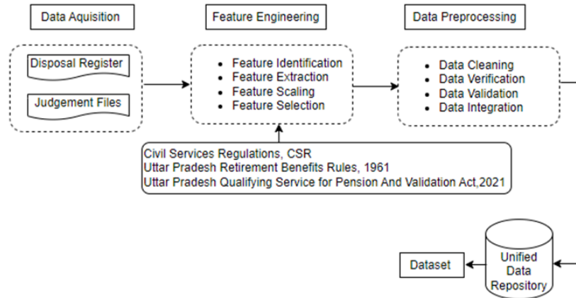
Fig.3: Dataset Preparation
