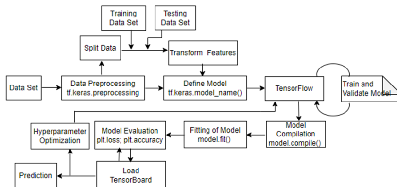
Fig.2: Research methodology
