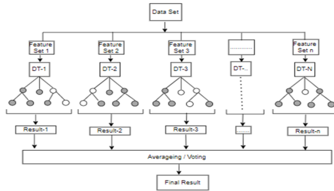
Fig.1: Decision Forest
