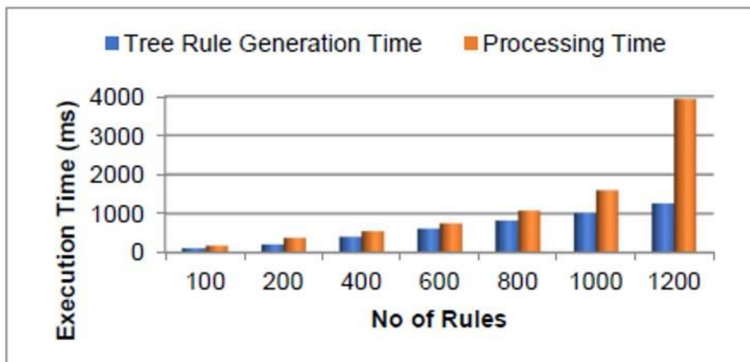
Figure 8 Execution Time for different numbers of rules
