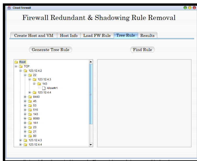
Figure 5 Altered Tree Generation
