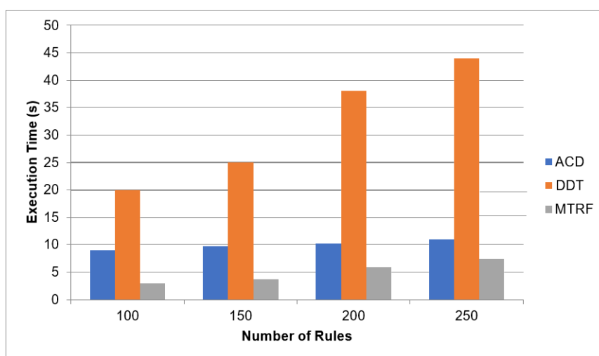
Figure 9 Total Processing Time Comparison
