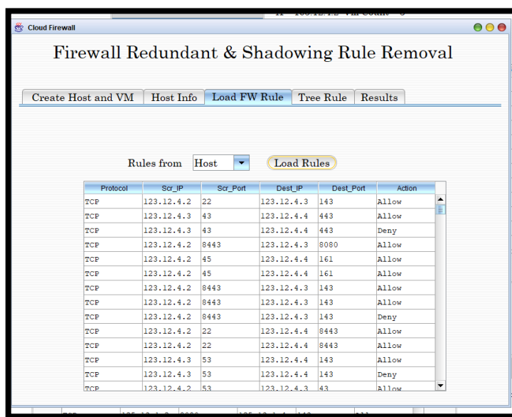
Figure 4: Firewall rules Loaded
