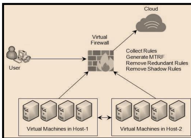
Figure 2 Altered Tree Firewall cloud Workflow
