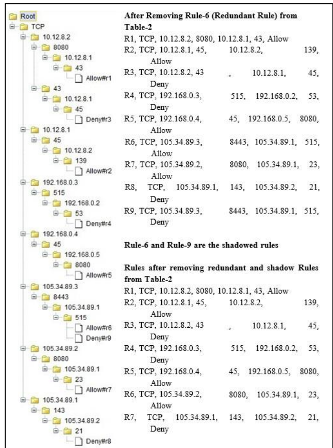
Figure 6 Tree Rules and Results
