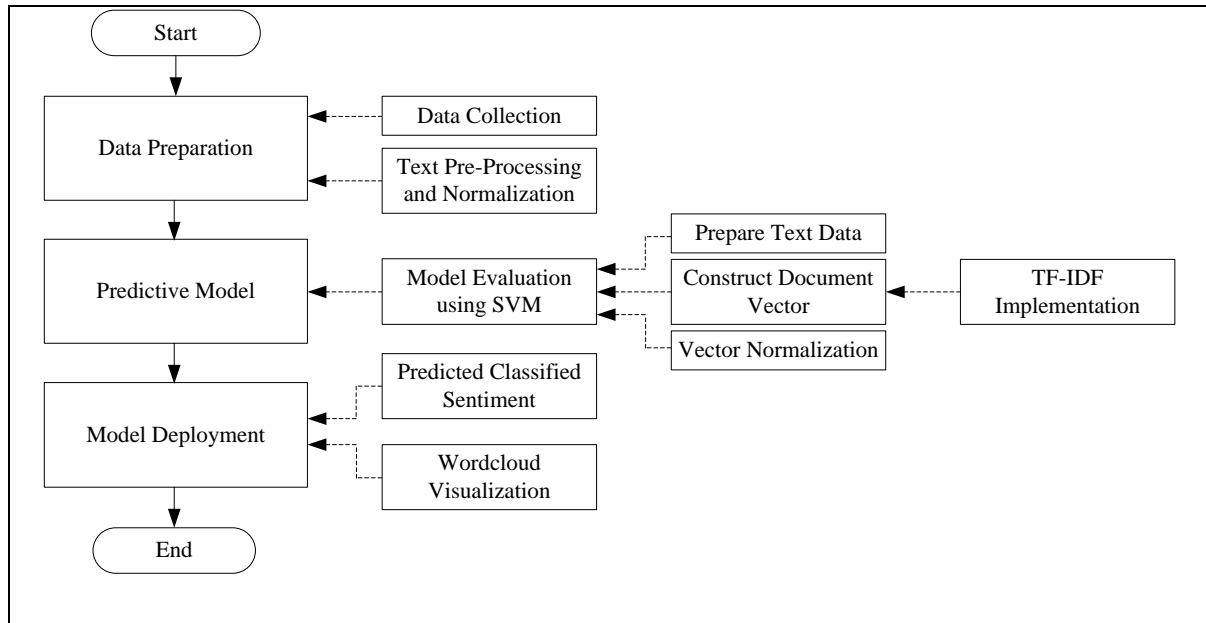
Figure 1. Back-end development phases for SAMIC
