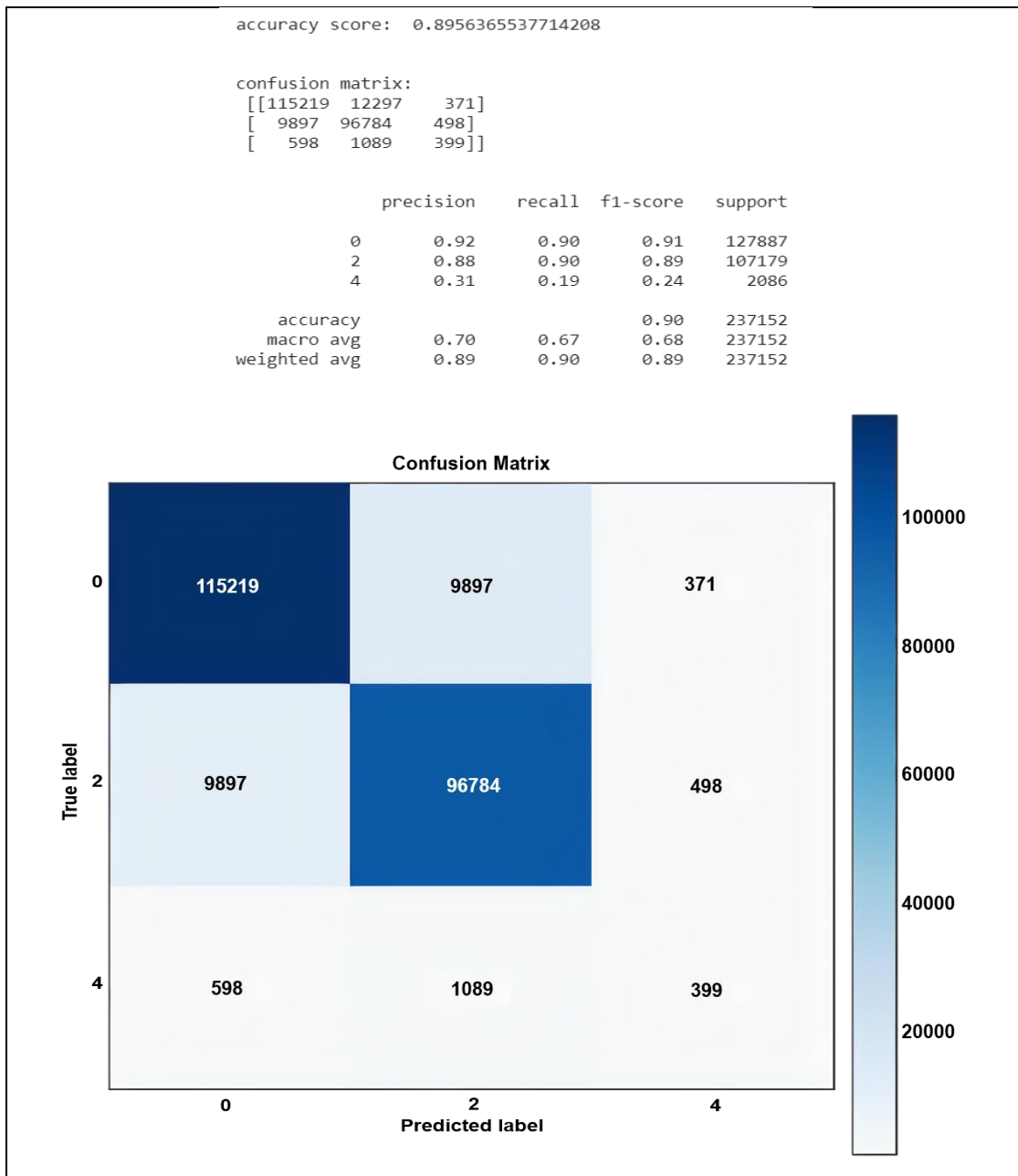
Figure 2. Confusion matrix of malay model
