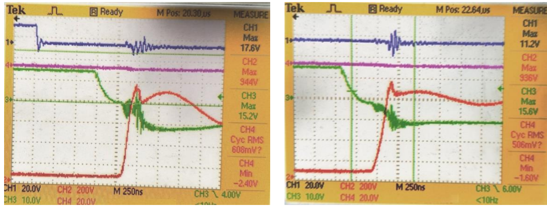
Figure 6: IGBT Collector voltage clamping
