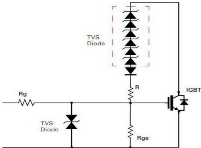
Figure 2: Dynamic collector voltage clamp using series connected Zener diodes.
