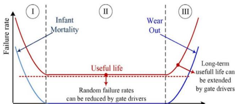
Figure 1: Typical failure rate during the lifecycle
