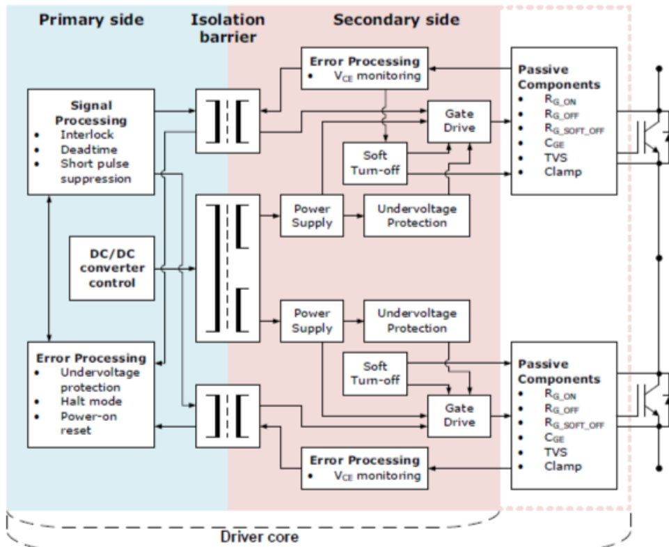
Figure 4: IGBT controller
