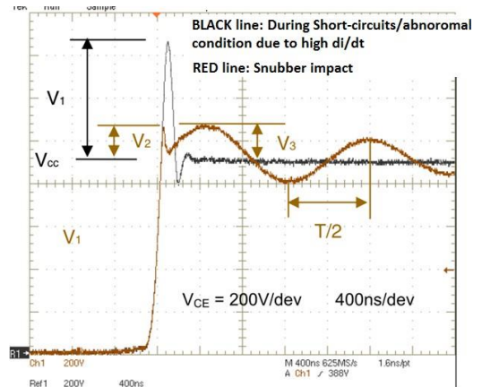
Figure 3: Switching characteristic during turned-off condition.
