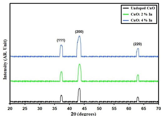
Fig.1. XRD-patterns.
