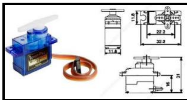
Fig 4: Servo motor (SG90)
