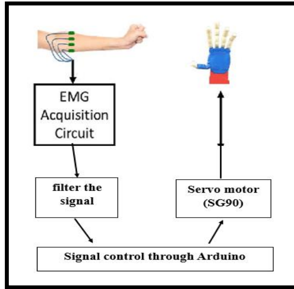
Fig 2: Block diagram of the proposed method for controlling prosthetic hands with raw EMG signals The prosthetic hand was designed using (Solid Work) software and printed on a 3D printer. Fig 3 shows prosthetic hand.
