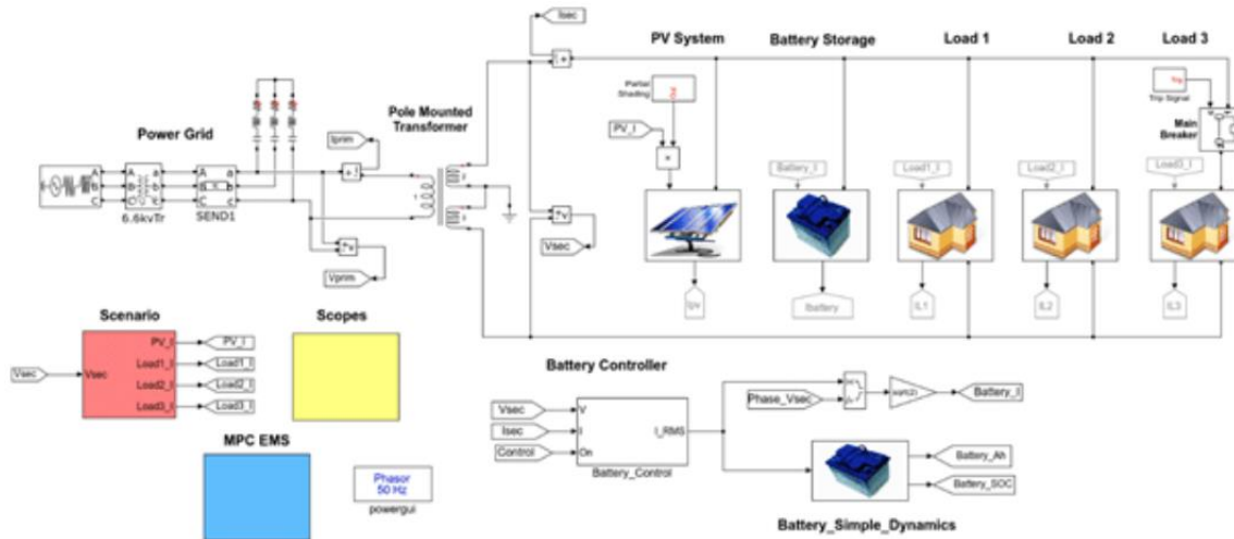
Figure 4: Simulink microgrid model
