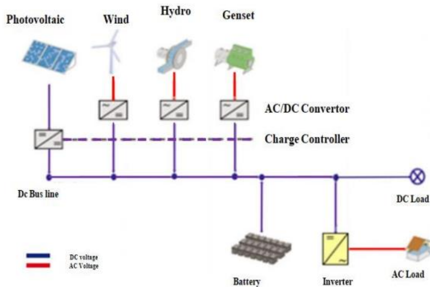
Figure 3-Renewable Energy Sources for Rural Electrification
