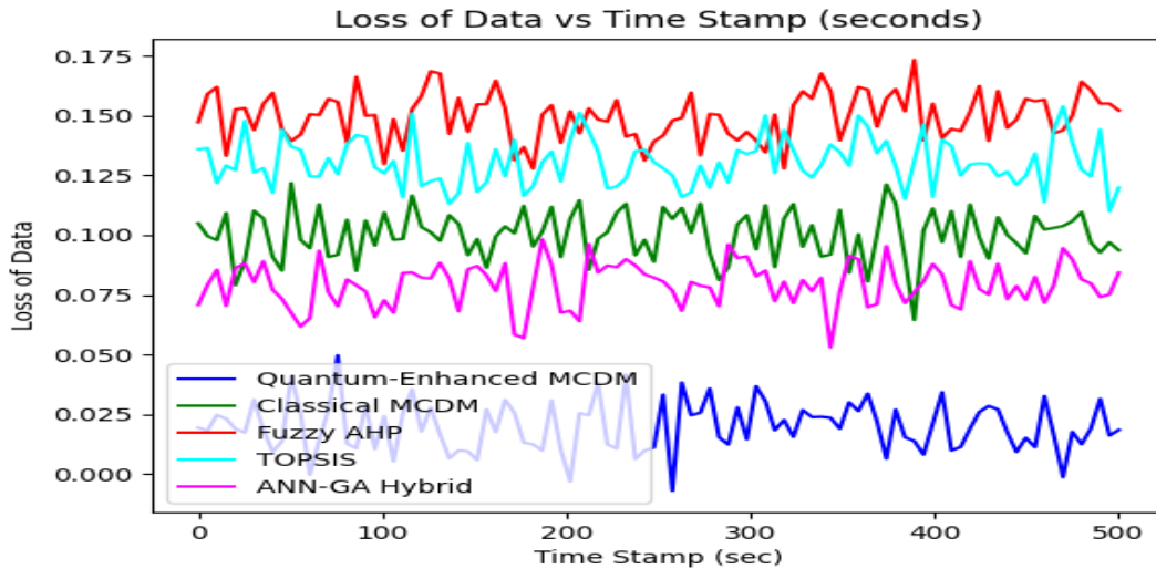
Figure 2. Loss of Data versus Time Stamp(sec)
