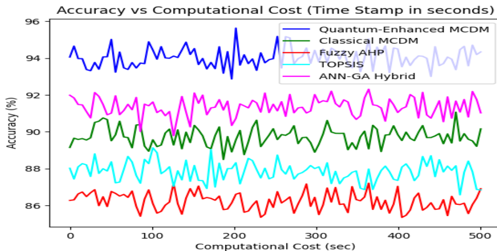
Figure 1. Accuracy (%) versus Computational Cost (sec)
