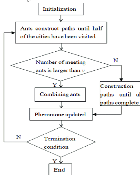
Fig 1: Ant Colony Algorithm.
