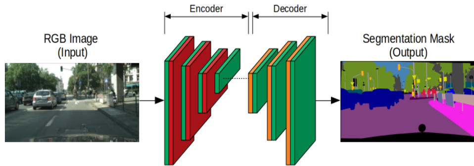
Fig 2: Image Segmentation.
