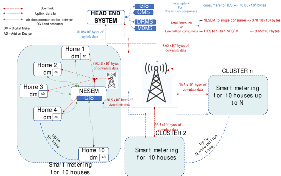
Figure 13: Decentralized framework uplink and downlink
