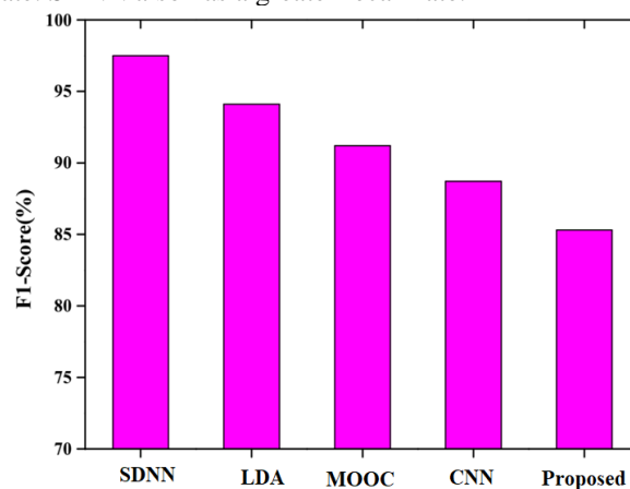
Figure 10: State-of-art result of F1-score
