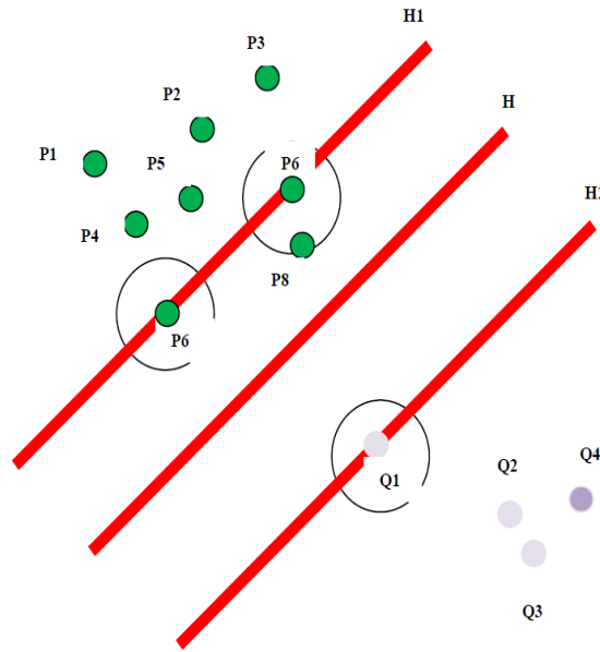
Fig 2: Hyperplane formation
