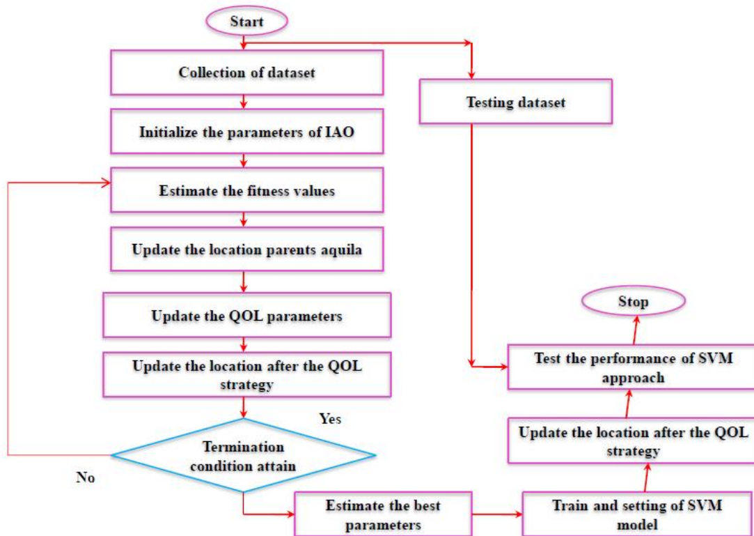
Fig 3: Schematic flow chart of our proposed work
