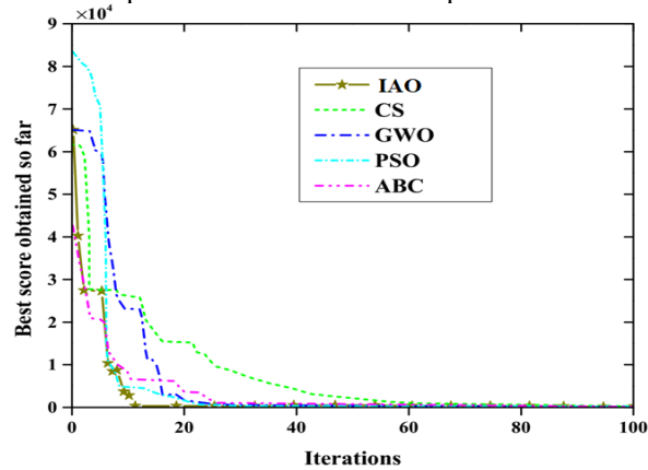
Figure 6: Convergence curve performance with respect to the state-of-art methods
