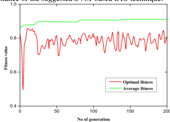
Figure 7: Performance analysis of proposed model with respect to fitness curve
