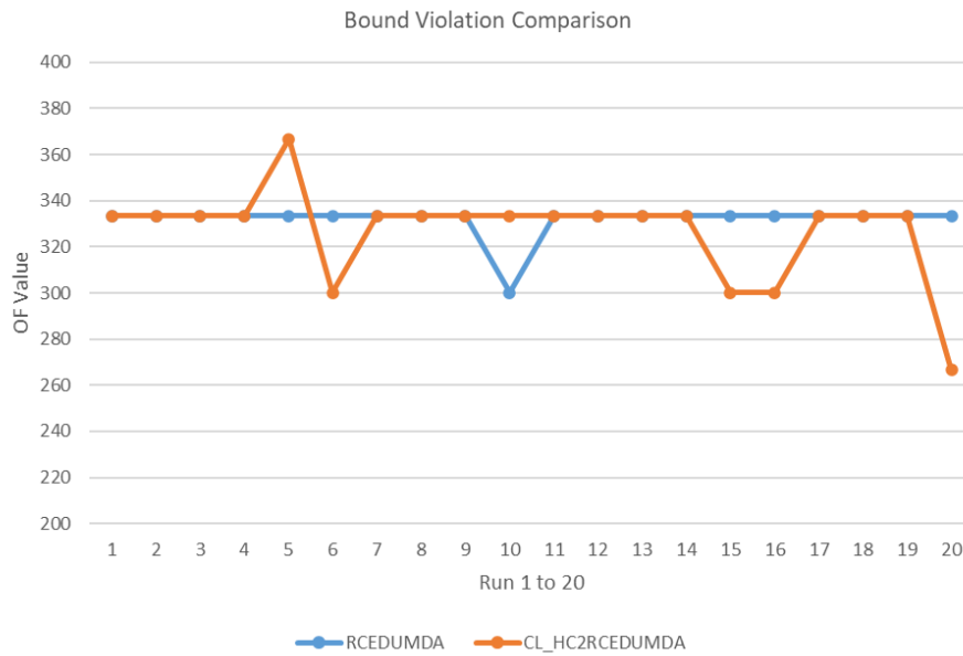
Fig.6. Bound Violations Comparison
