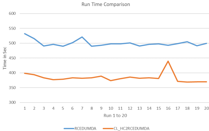
Fig.7. Run Time Comparison
