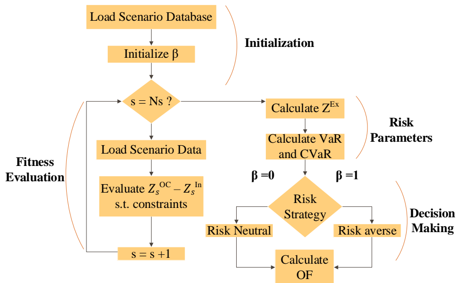
Fig. 1 Fitness Function Evaluation
