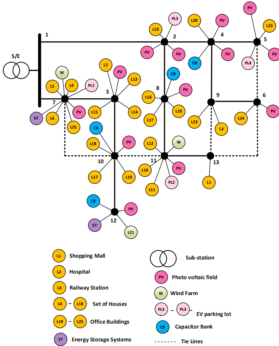
Fig.4. 13-Bus network system [11]
