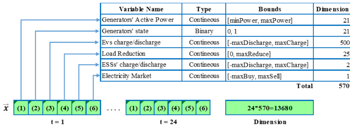
Fig. 2. Solution Vector of ERM
