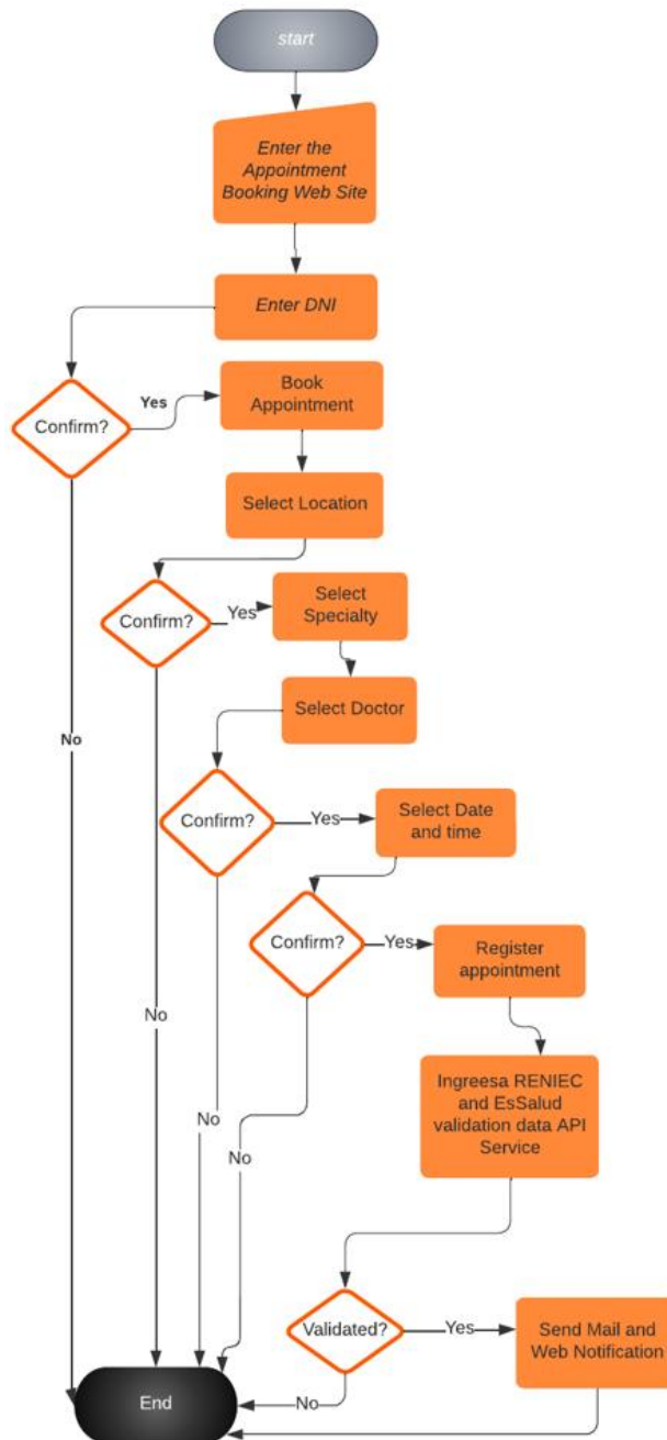
Figure 1. Appointment Reservation Flow Diagram
