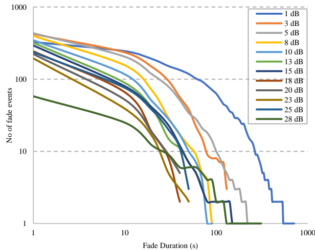
Fig 6: Total number of fades of duration exceeding threshold
