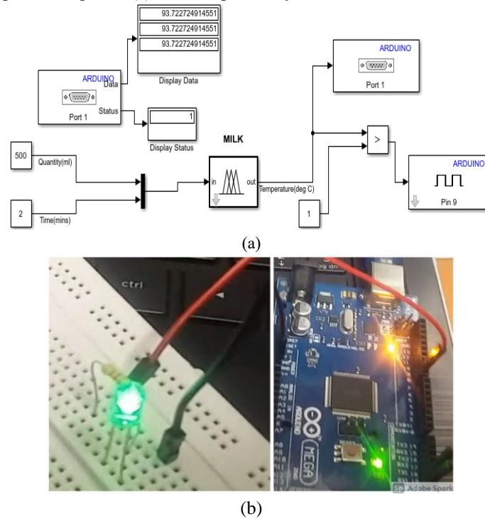
Figure 5 (a) “Hardware in Loop” for type Milk (b) Hardware Independency Testing for Milk.
