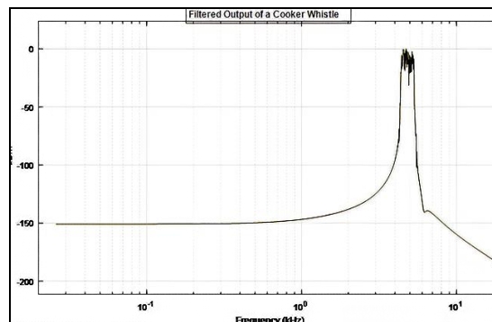
Figure 4 Spectrum of Filtered Cooker Whistle Audio Sample.
