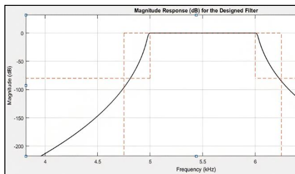
Figure 3 Magnitude Response for the Designed Cooker Whistle Identification Filter.
