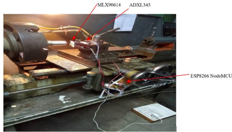
Figure 2 - Placement of sensor on the lathe machine
