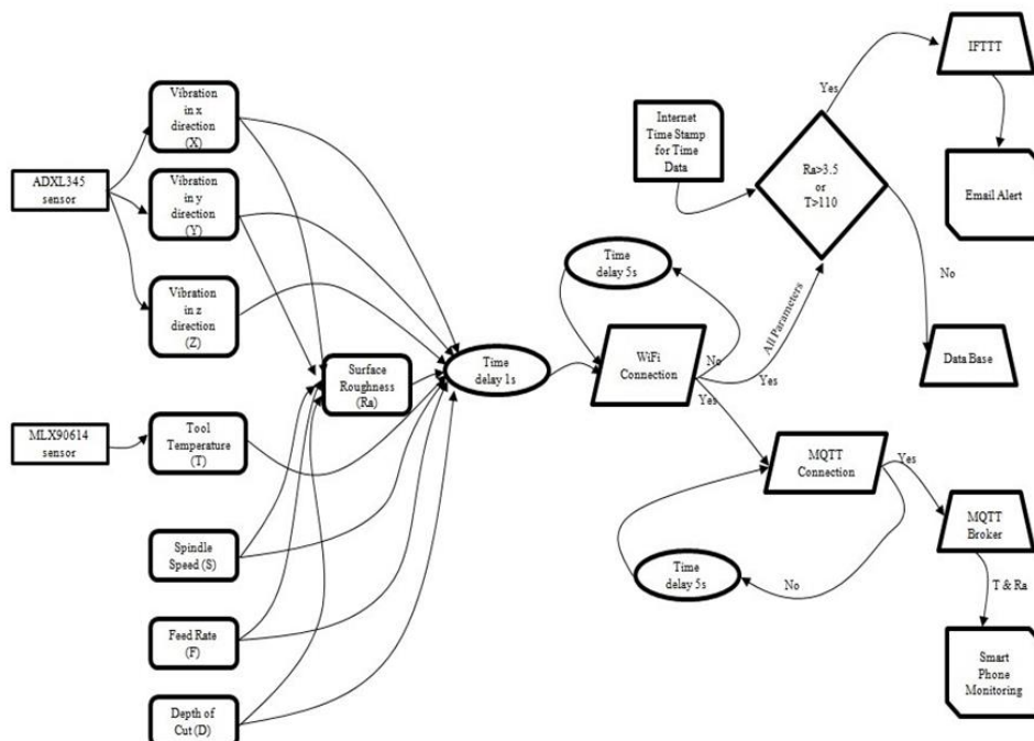
Figure 5 - Network of IoT system operation, modified from [19]
