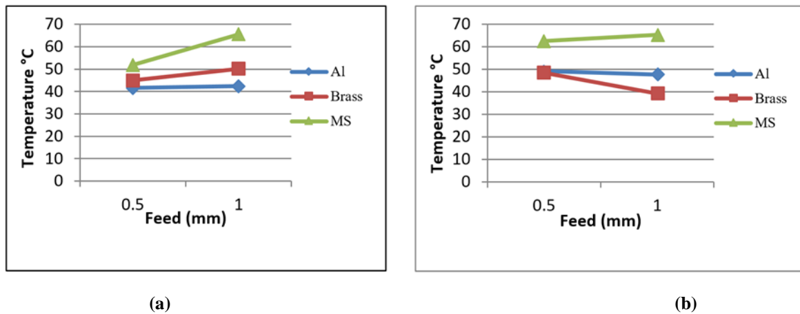
Fig. 7 (a) Feed Vs Temperature for S=350rpm and D=0.5mm (b) Feed Vs Temperature for S=500rpm and D=0.5mm
