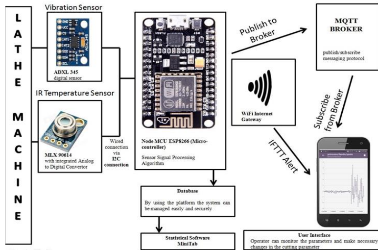
Figure 4 - IoT system design layout as modified by [19]
