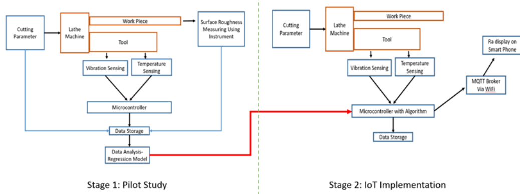
Figure. 3 – Schematic diagram of the experimental study analysis procedure
