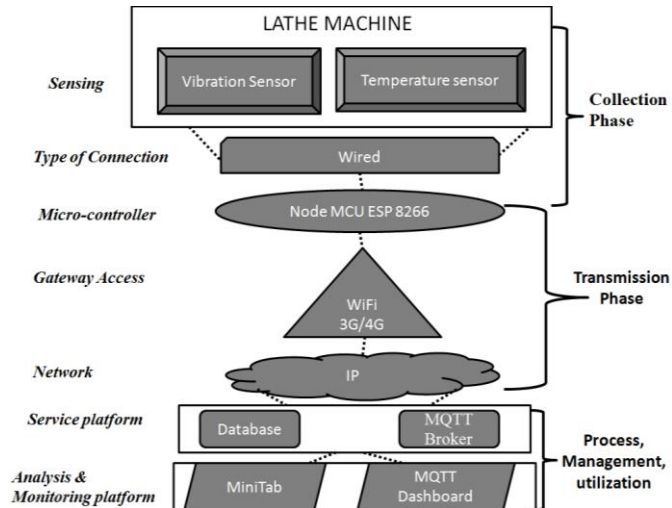
Figure 1 - Vertical representation of the experimental setup and its phases as modified by [18]
