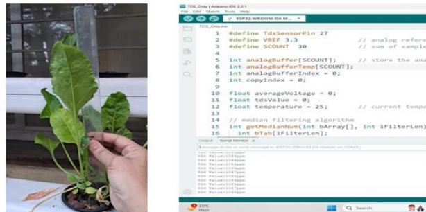
Figure 12 (a) plant growth at 1090ppm Figure 12(b) Serial monitor: TDS approximately 1100ppm With all the parameters within required range- pH= 6, TDS = 1100-1200 ppm and environmental temperature = 25 o C, the plant growth and the root growth is shown in fig 13 (a and b) . It was observed that the plant appearance was fresh green rather than other plant appearances with changes parameters.
