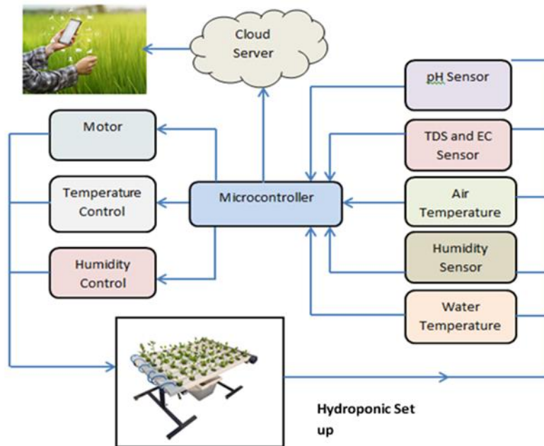
Figure 2 IoT System Architecture for Hydroponic Set Up
