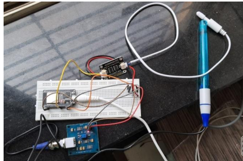
Figure 1 Proposed Circuit for pH and TDS sensing
