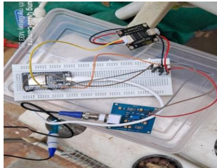
Figure 3 Sensor Network in the hydroponic set up
