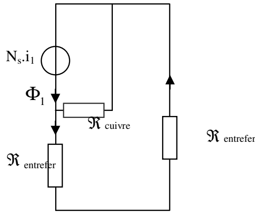
Figure 7: Network reluctance modeling inductance
