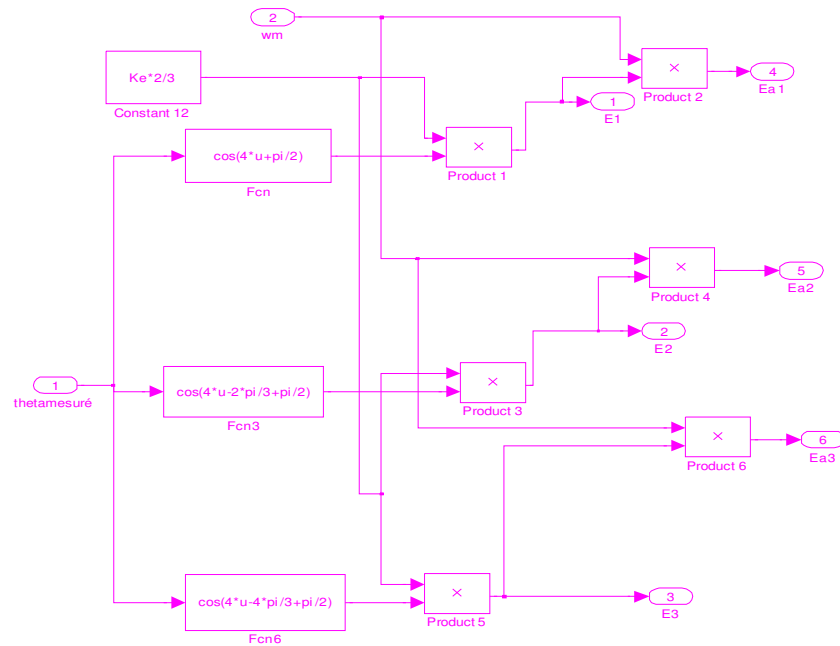
Figure 14: Model Simulink of the back electromotive forces
