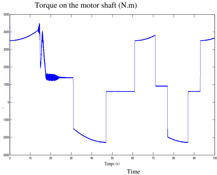
Figure 20: Torque on the motor shaft
