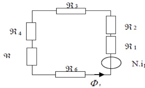
Figure 9: Reluctance network modeling the mutual inductance
