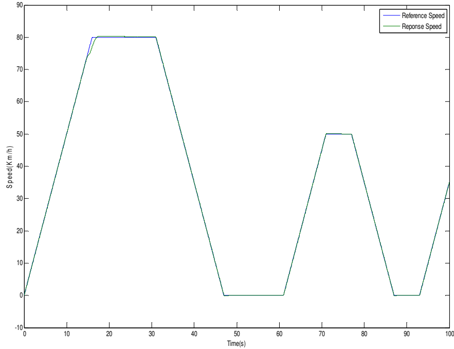
Figure 18: Speed response
