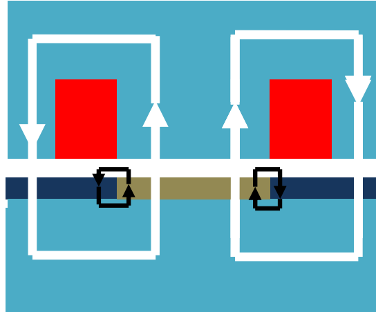
Figure 5: Distribution of the field lines to a position of maximum recovery
