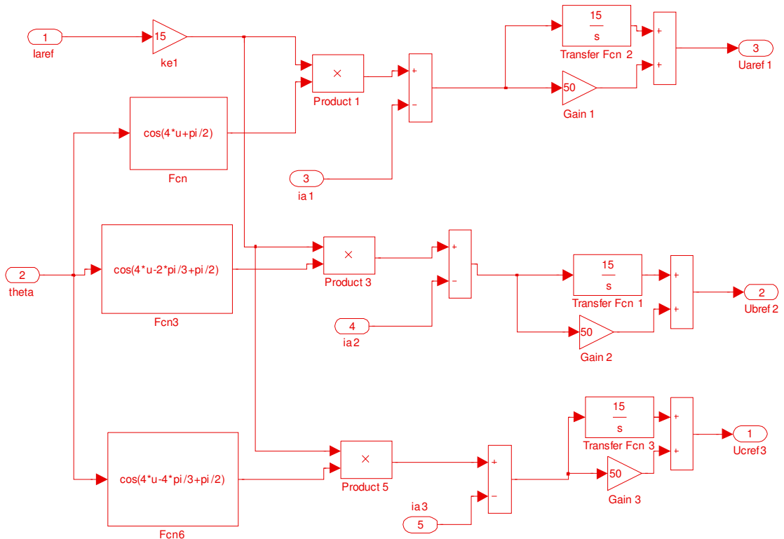
Figure 13: Simulink model of currents regulators
