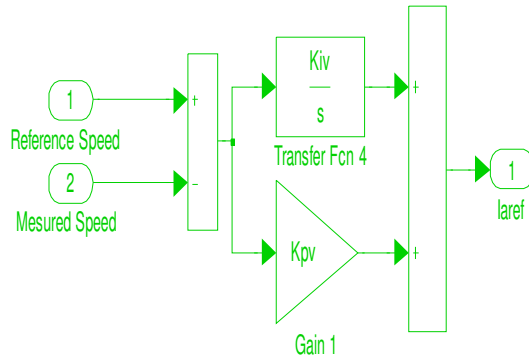
Figure 12: Simulink model of the speed regulator
