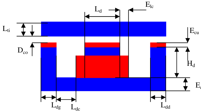
Figure 2: Design parameters of the generator coil
