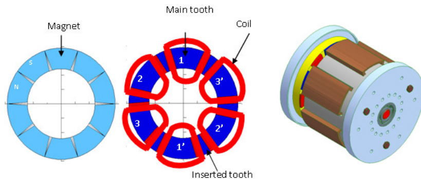
Figure 4: Configuration to 5 pairs of poles and 6 main teeth
