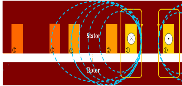
Figure 8: Distribution of the flux generated by the coil powered and captured by the adjacent coils
