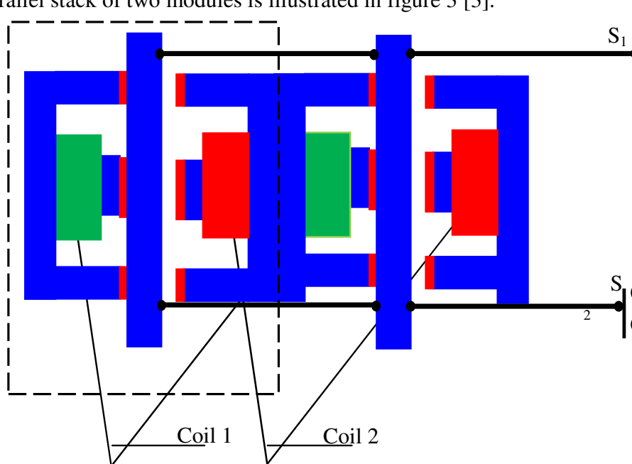
Figure 3: Stacking in parallel of two modules
