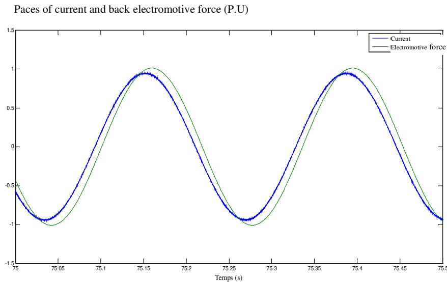
Figure 22: Paces of current and back electromotive force
