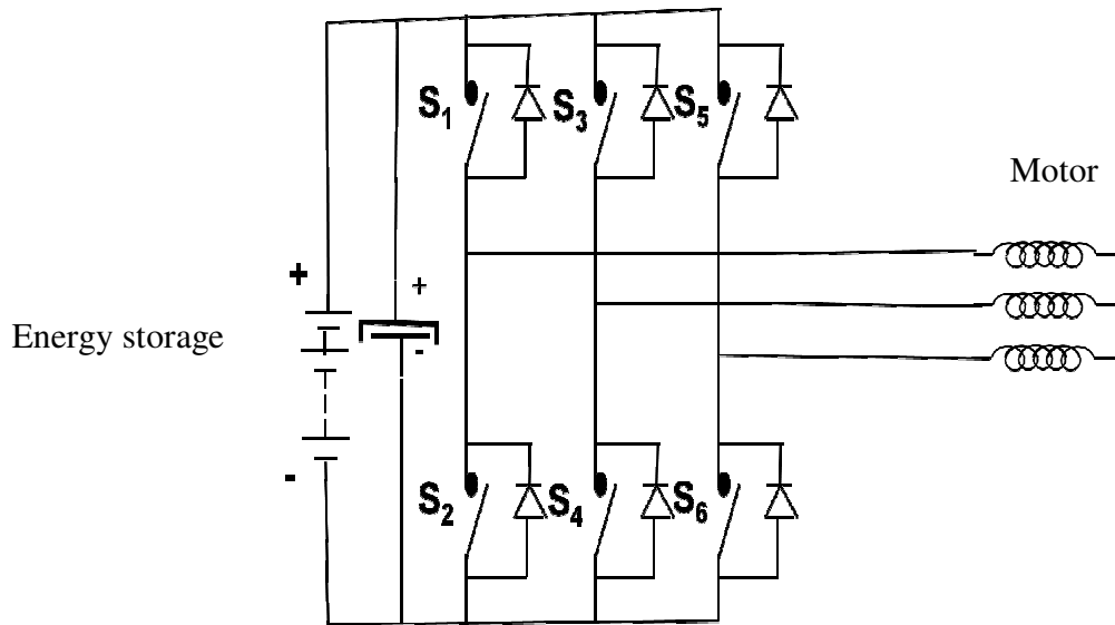
Figure 1: Power chain structure
