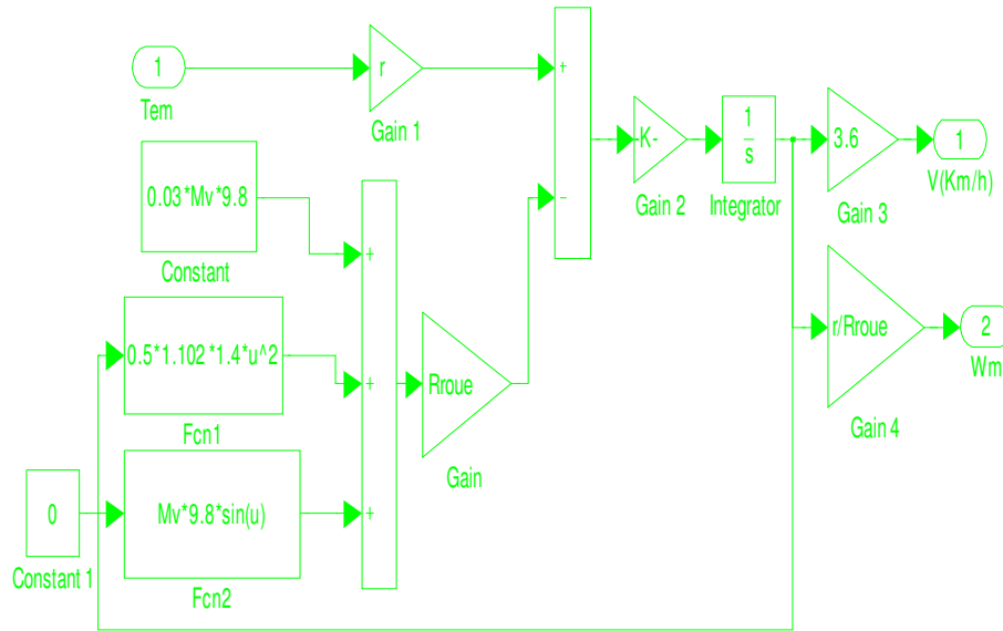
Figure 16: Simulink model of the dynamic equation
