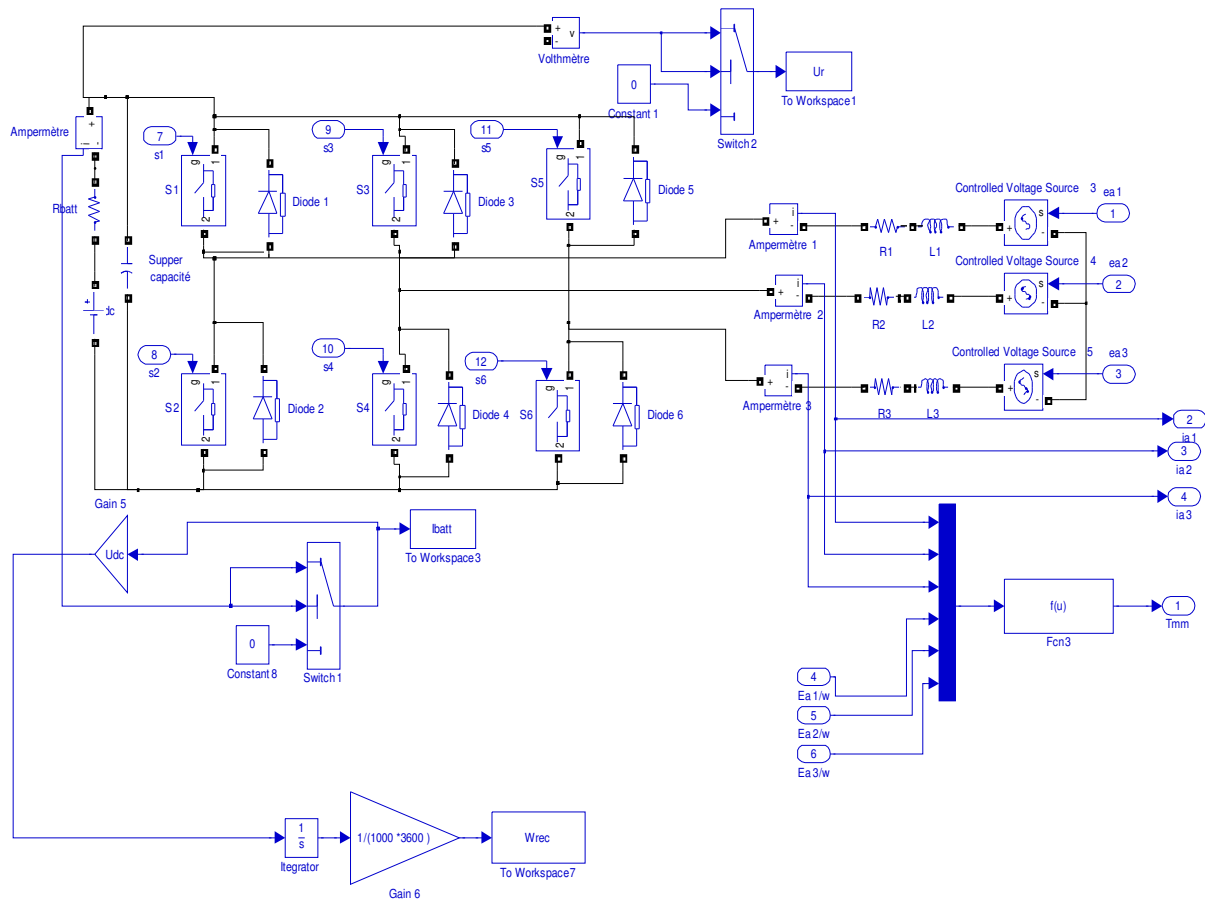
Figure 11: Simulink model of the motor-converter
