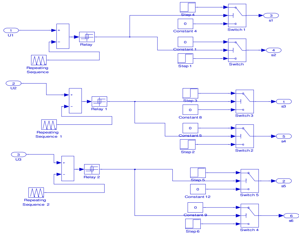
Figure 15: Simulink model of control signals generator
