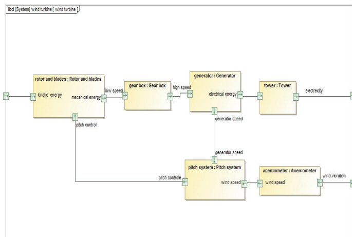
Fig. 7. Internal block diagram.
