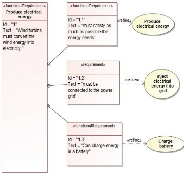
Fig. 3. Functional requirement diagram.
