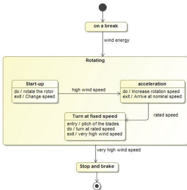
Fig.8. State machine diagram.
