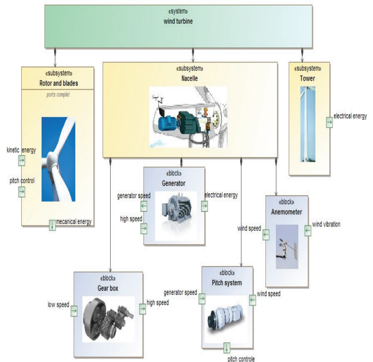
Fig.6. Block definition diagram.
