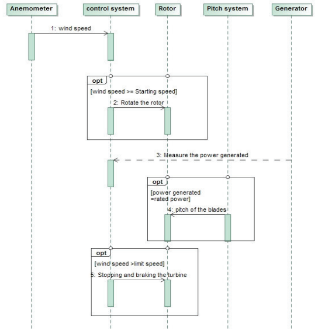
Fig. 5. Sequence diagram.
